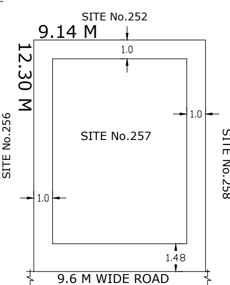
SITE PLAN
